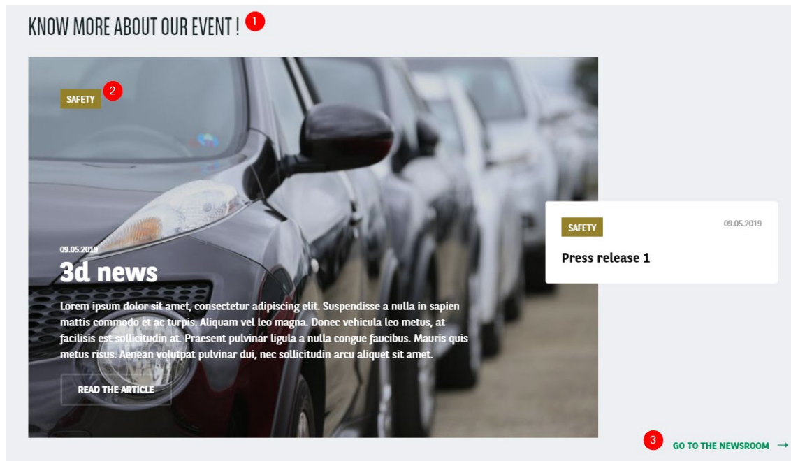
With theme
