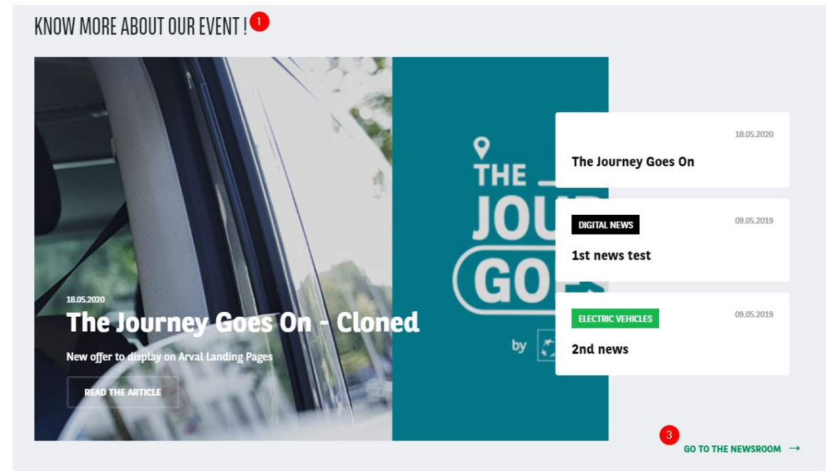
Without theme
